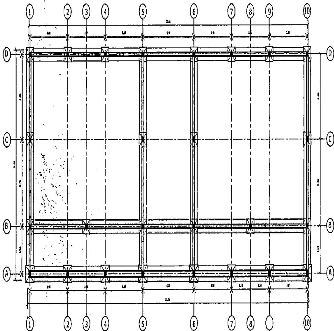
FOUNDATION PLAN
