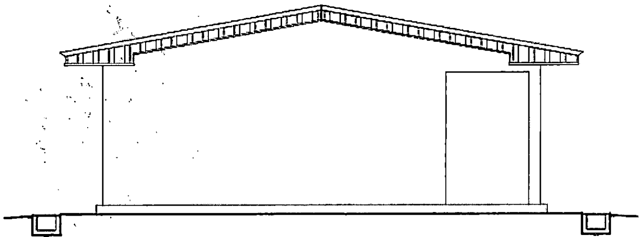
LEFT ELEVATION
